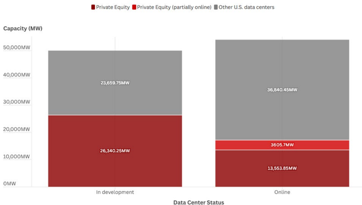
Figure 1. Capacity of private equity-backed data centers and other U.S. data centers, by status (as of December 2025)
