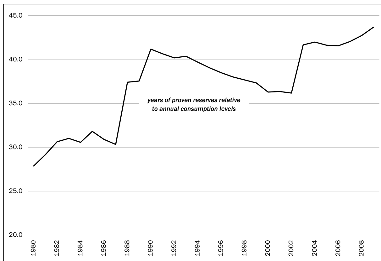
Figure 6. Ratio of barrels of proven reserves to barrels of annual consumption, 1980-2009
